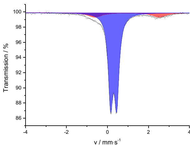
Fig. 8 Mössbauer spectrum of [\text{Fe}(\text{Htrz})_2(\text{trz})](\text{BF}_4) \cdot \text{H}_2\text{O} at 293 K
