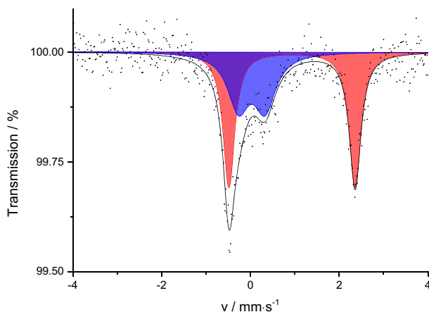
Fig. 4 Mössbauer spectrum of [\text{Fe}(\text{NH}_2\text{-trz})_3](\text{BF}_4)_2 in PLA Fibers at 293 K
