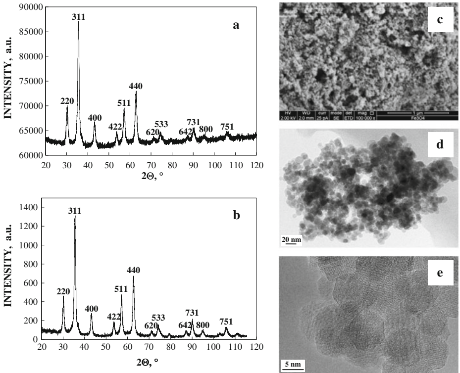
Fig. 1 X-ray diffraction patterns of as-prepared Fe 3 O 4 (a) and Fe 3 O 4 -CO (b) samples, SEM (c), TEM (d) and high-resolution TEM (e) images of as-prepared Fe 3 O 4
