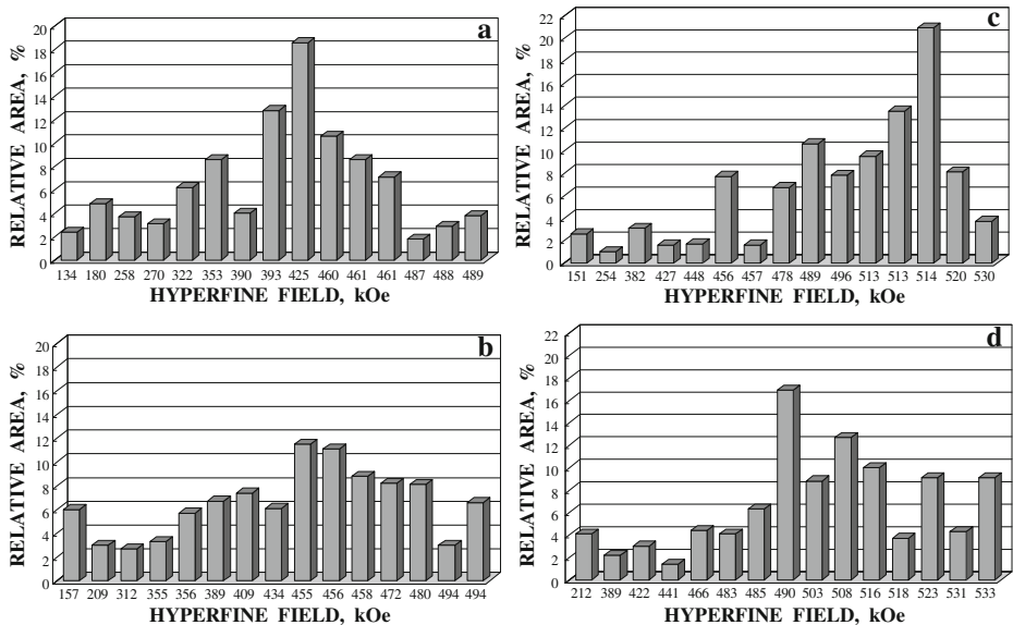
Fig. 4 Histograms of the relative areas of magnetic sextets obtained from the better fits of Mössbauer spectra of as-prepared Fe 3 O 4 (a, b) and Fe 3 O 4 -CO (c, d) samples measured at 295 K (a, c) and 90 K (b, d)
