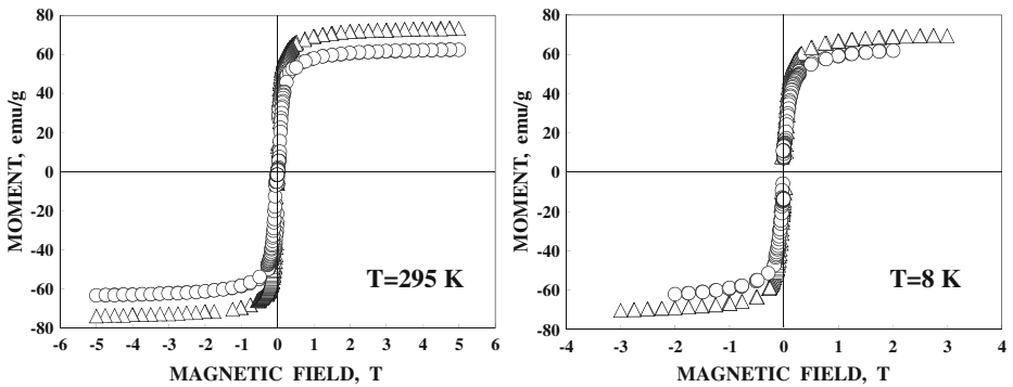
Fig. 2 Magnetization curves for Fe 3 O 4 (○) and Fe 3 O 4 -CO (△) measured at 295 and 8 K. The mass for Fe 3 O 4 in the sample of Fe 3 O 4 -CO was determined using TG measurement
