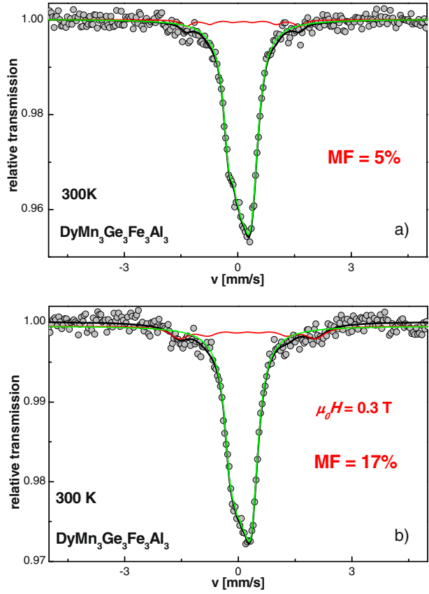
Fig. 2 The Mössbauer spectra of \text{DyMn}_3\text{Ge}_3\text{Fe}_3\text{Al}_3 sample measured at 300 K without (a) and with applied magnetic field (b) of induction \mu_0 H = 0.3 T
