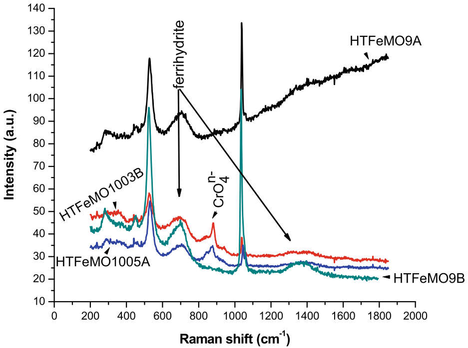
Fig. 3 Raman spectra of the hydrotalcites before and after Cr (VI) sorption at pHs 3 and 5
